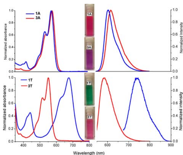
Figure 2. Absorption (left) and emission (right) spectra of anthracene-based 1A/3A (top) and tetracene-based 1T/3T (bottom) in \text{CH}_2\text{Cl}_2 . The insets show photographs of \text{CH}_2\text{Cl}_2 solutions of 1 and 3 .
