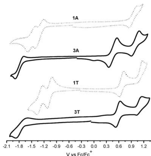
Figure 4. Cyclic voltammograms of quinones 1 and arylated compounds 3 in 0.2 M Bu 4 NPF 6 in CH 2 Cl 2 .
