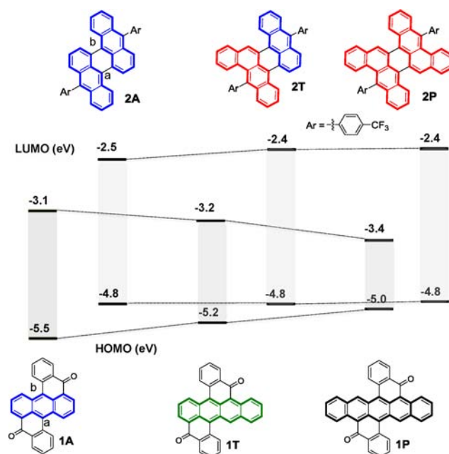
Figure 3. DFT-calculated HOMO–LUMO energies of quinones 1 and their corresponding aromatics 2 .
