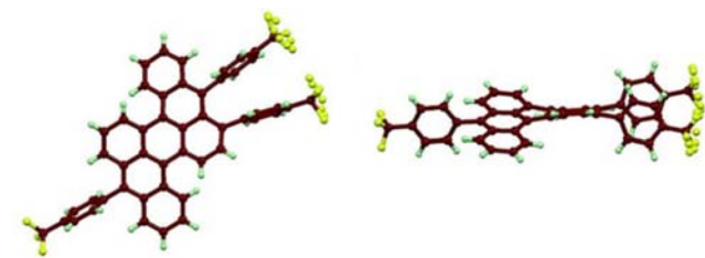
Figure 1. Crystal structure of 3A .
