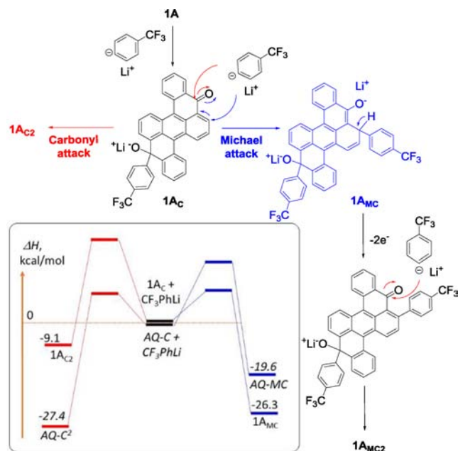
Scheme 2. Proposed Mechanism of Arylation of 1A ; the Inset Shows the DFT-Calculated Energy Diagram for Michael/Carbonyl Addition to 1A in Comparison with 9,10-Anthraquinone (AQ)
